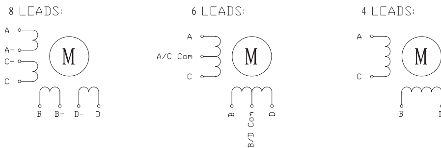
1. Bipolar (parallel) connection
