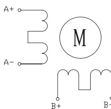
2. Bipolar (series) connection
