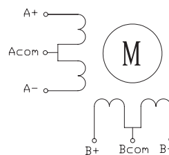
3. Unipolar connection
