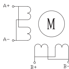
1. Bipolar (parallel) connection
