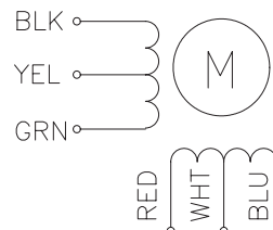
6 LEADS
