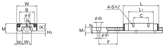
Modelos RSR7 a 12N/7M/9KM/12VM
