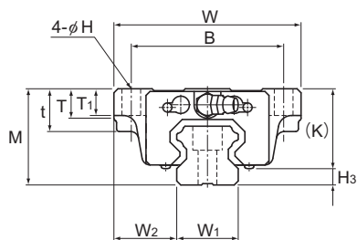
Modelos HSR15, 25 a 35M1B/M1LB
