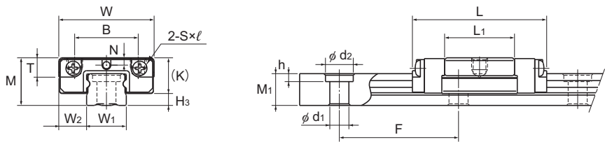
SRS5M
