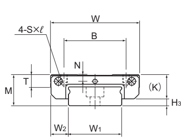
Modelos SRS7WM/9, 12WM/WN
