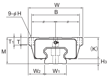
Modelos HSR100 a 150HB
