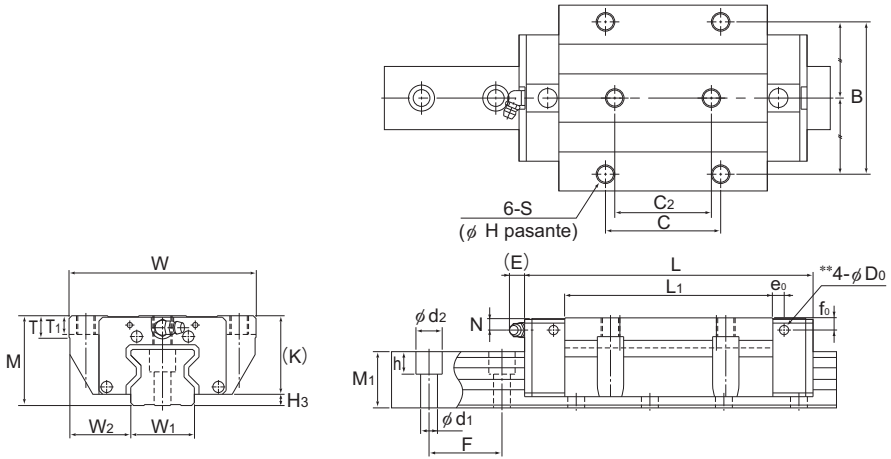
Modelos SRG25 a 65C/LC
