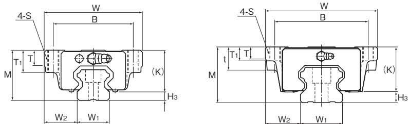
Modelos HSR15 a 35A/LA/AM/LAM
