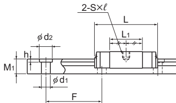
Modelos RSR5M/5TN
