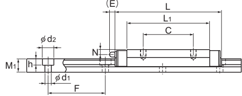
Modelos RSR15WV/WVM/WN
