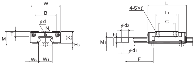
Modelos RSR7 a 12ZM
