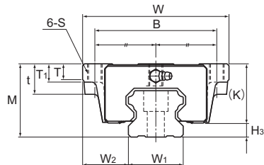
Modelos HSR45 a 85CA/HA
