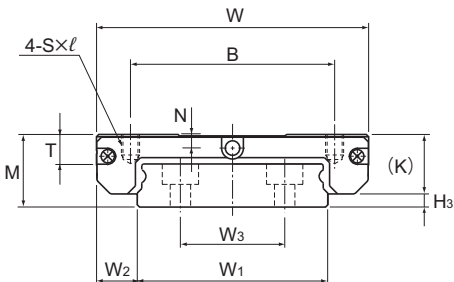
Modelos SRS15WM/WN
