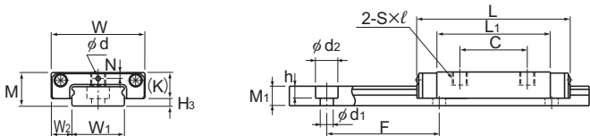
Modelos RSR3 a 7WM/WN
