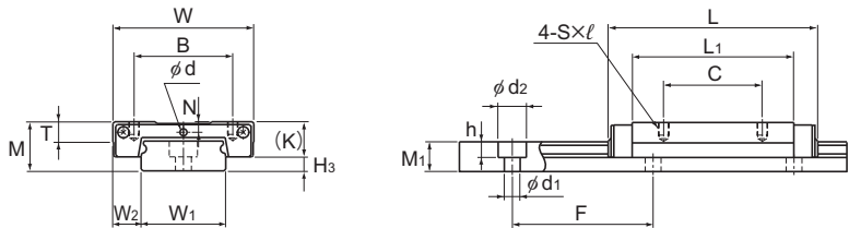
Modelos RSR9, 12WV/WVM/WN
